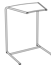
Magnes II 300 Dimensions 410w×330d mm Writing tablet height 536 mm
