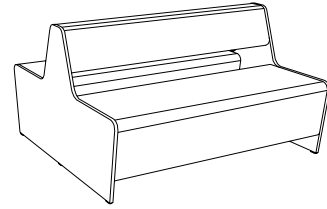
Magnes II 502 Dimensions 1330w×1260d mm Back height 780 mm Seat height 440 mm
