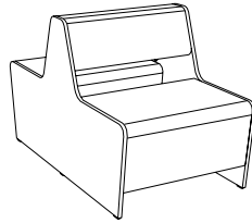
Magnes II 501 Dimensions 670w ×1260w mm Back height 780 mm Seat height 440 mm
